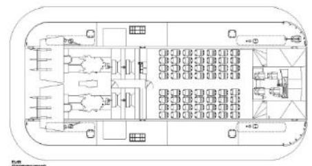
Passenger Configuration Non Statutory Compliant (56 seats)
